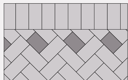
Alternative recommendation – insertion of pavers cut to three quarter length.
