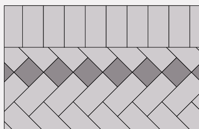
Recommended insertion of pavers cut to half length.
