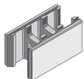
400x190x200mm
