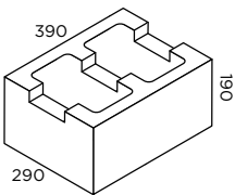
30.42TB Trough Block 18.2kg 60 per pallet 1092kg pallet weight
